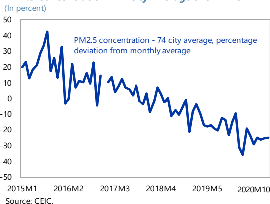
PM2.5 Concentration - 74 City Average over Time
